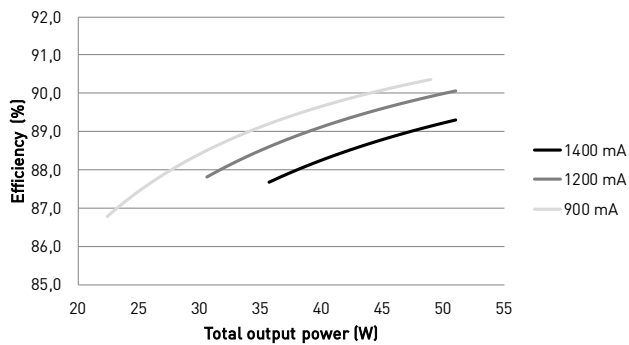
Typical efficiency
