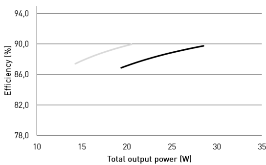
Typical efficiency
