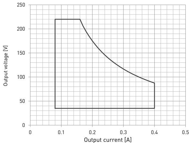
From 80 mA to 400 mA, full dimming range ( 1 % - 100 %) available in the whole area.
