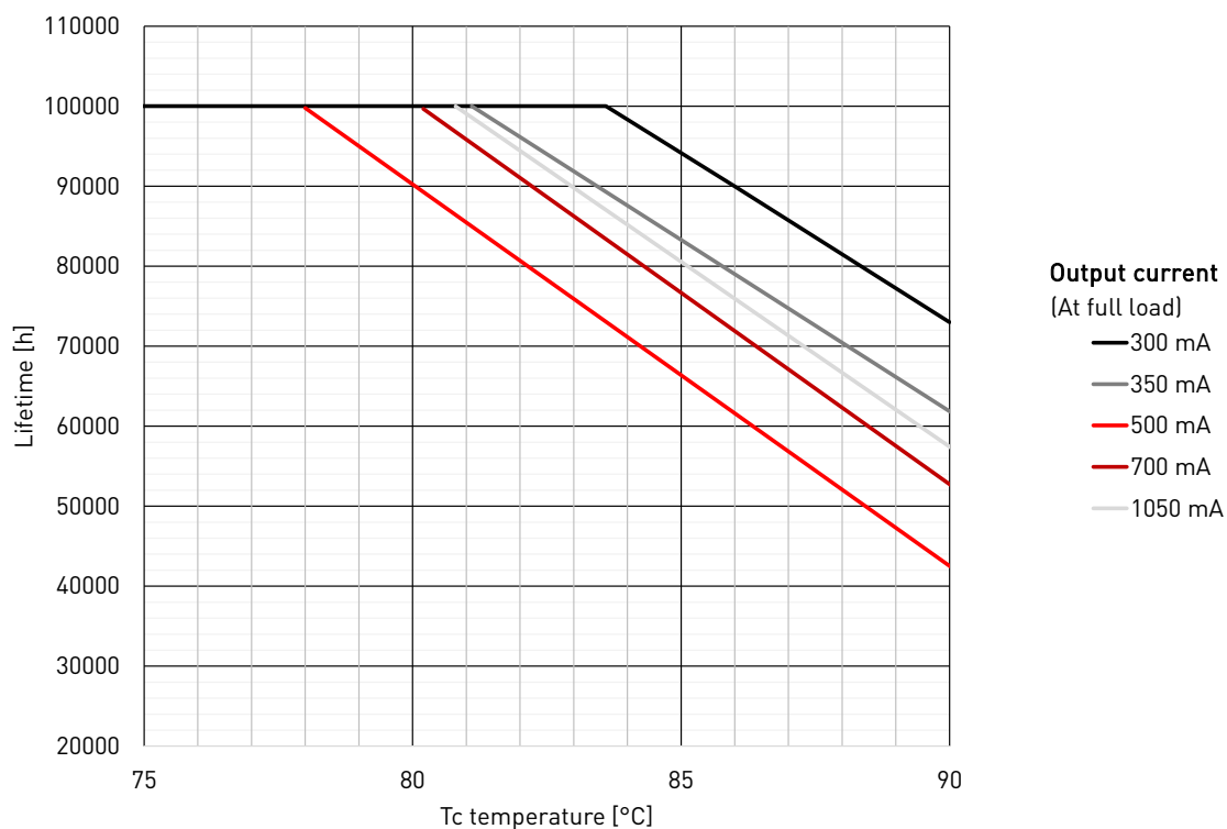
Lifetime estimations in built-in use, reference conditions
