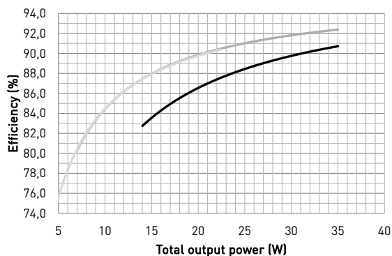
Typical efficiency
