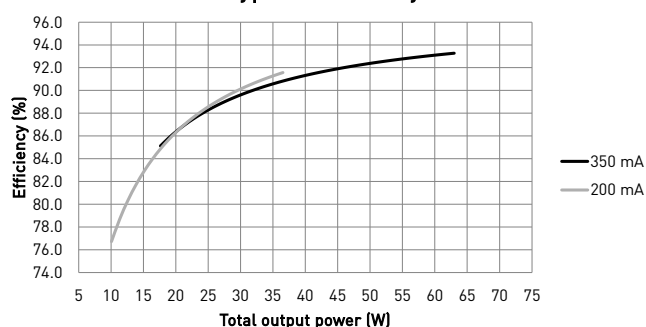
Typical efficiency
