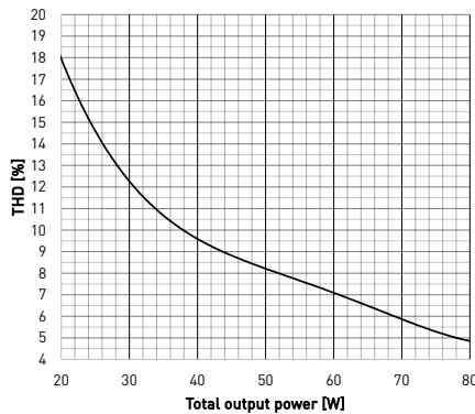
Current THD
