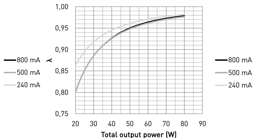
Typical power factor
