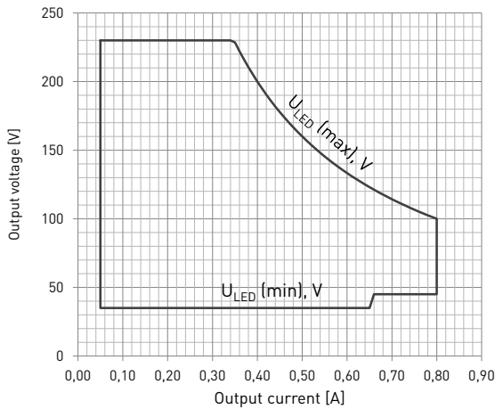
250 V Uout mode, default
