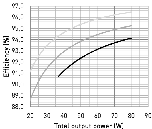
Typical efficiency
