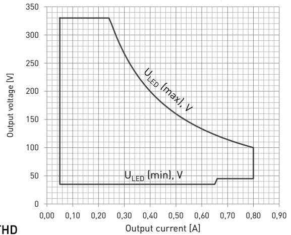
350 V Uout mode, enabled only via NFC
