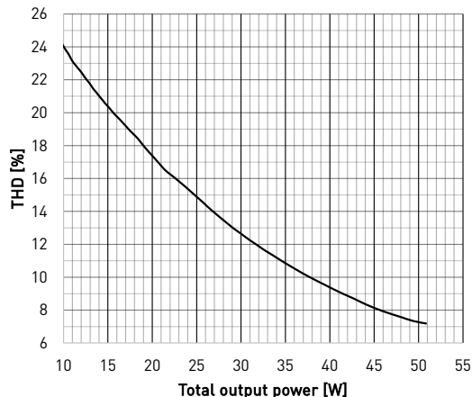
Current THD
