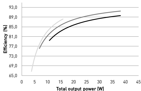
Typical efficiency
