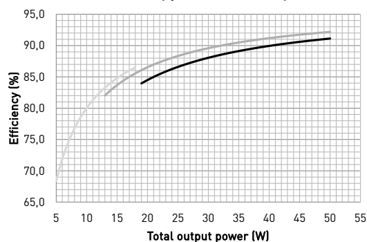
Typical efficiency
